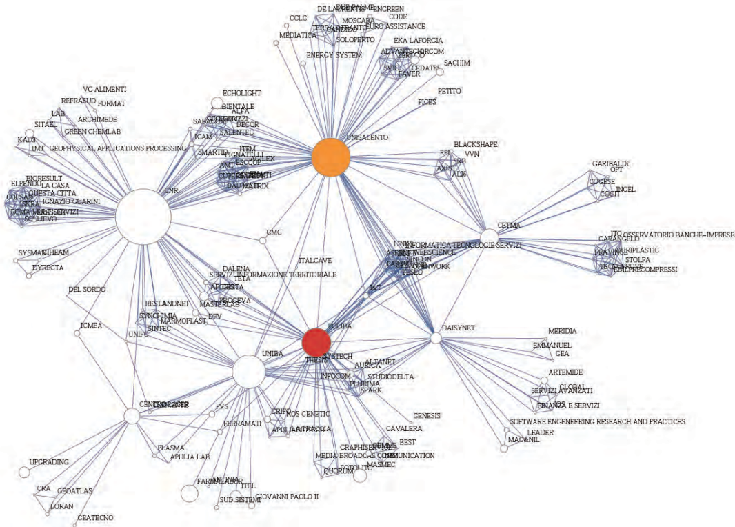
Figura 30: Network analysis.
